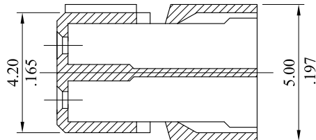
SEC.:A-A
