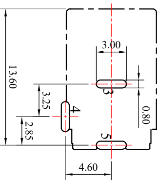
Recommended P.C.B Layout General Tolerance:±0.05
