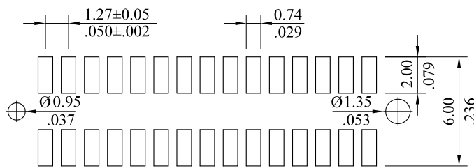
RECOMMENDED HOLE PATTERN
