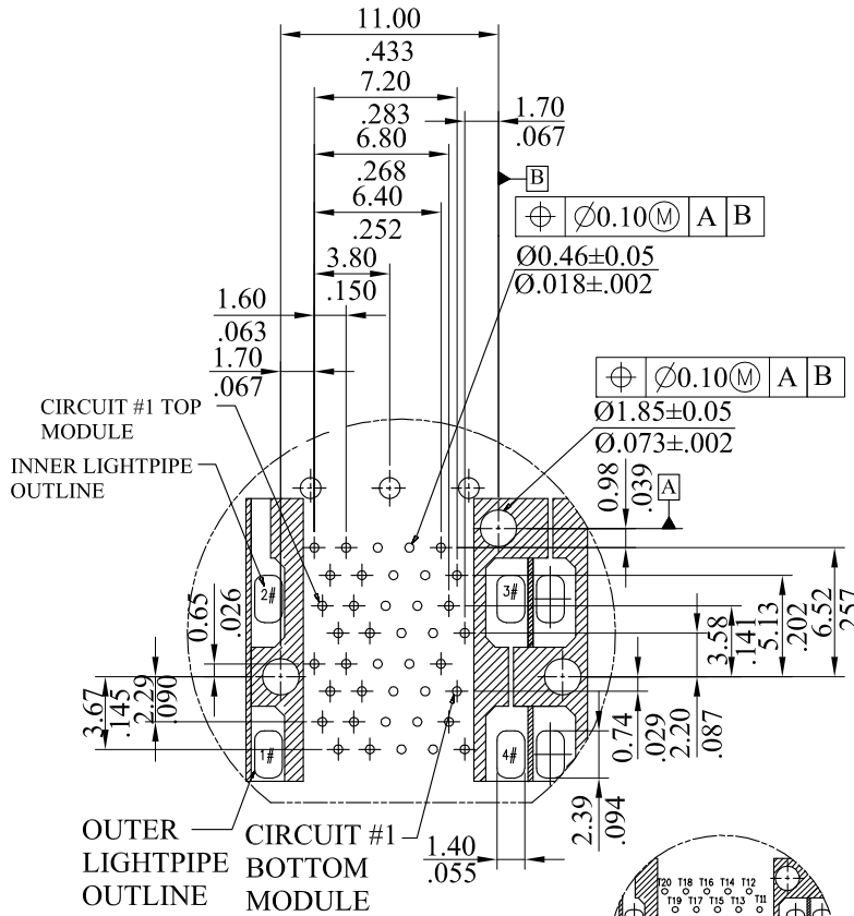
DETAIL A SCALE 2:1 PCB LAYOUT
