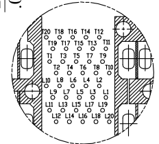
CONNECTOR PIN-OUT COMPONENT SIDE OF BOARD
