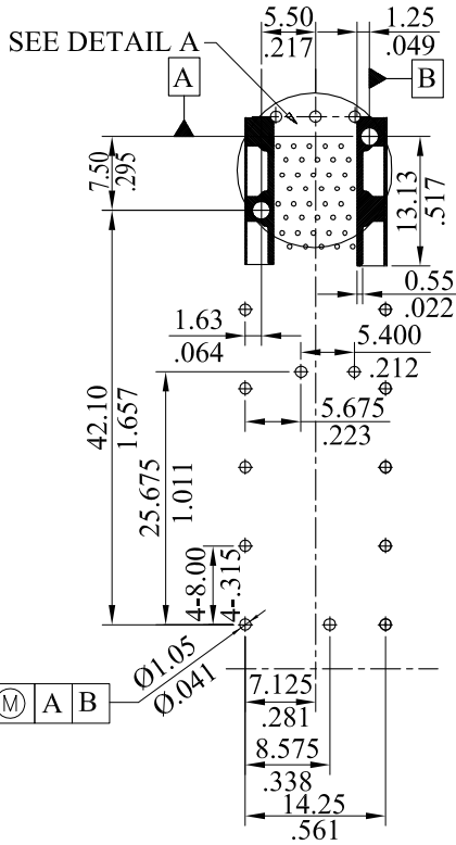
BEZEL CUT-OUT CENTER SPACING DETAIL BEZEL THICKNESS: 0.8-2.6
