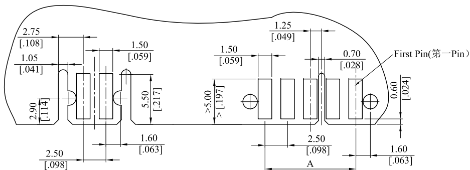
PCB LAYOUT
